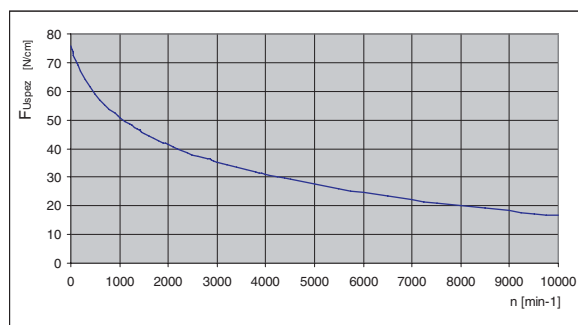
Tooth shear strength / rpm
