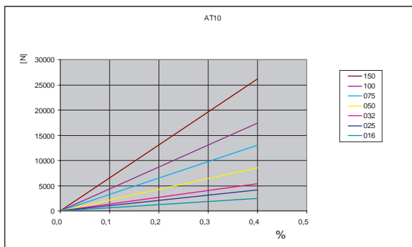
Load / Elongation [ % ]
