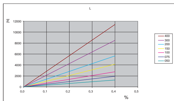
Load / Elongation [ % ]
