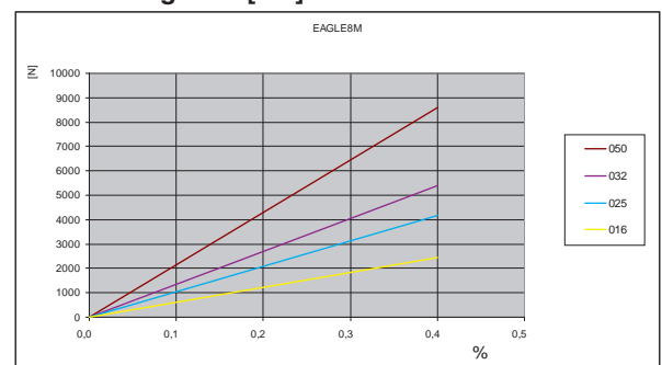
Load / Elongation [ % ]
